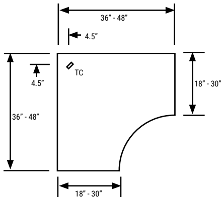
Corner Worksurfaces - 1 Piece
